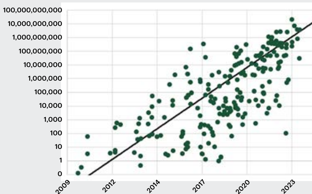
Figure 1: Computation used to train notable AI systems (measured in petaFLOP, log scale)
